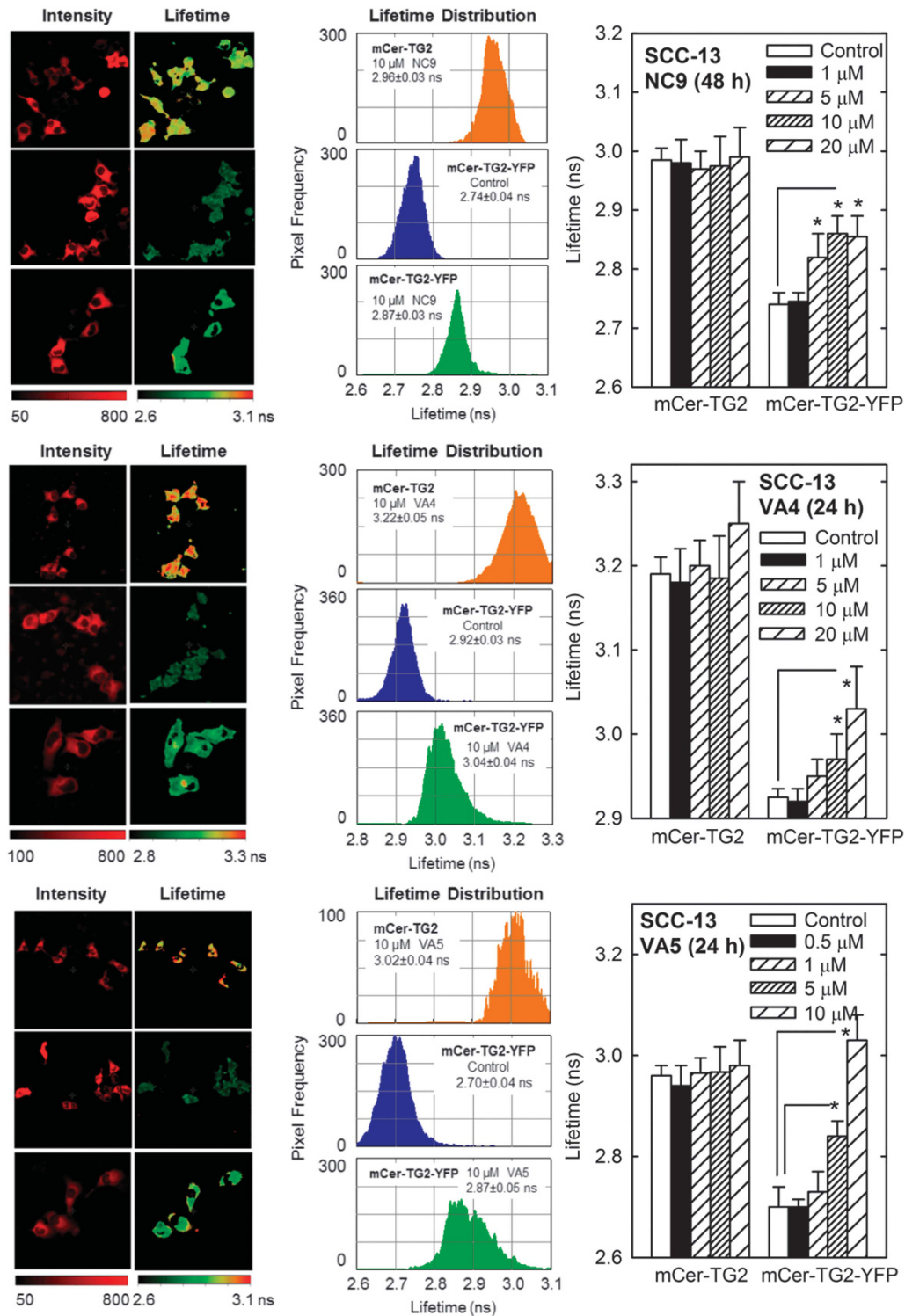
Figure 2. Irreversible TG2 transamidase site-selective inhibitors shift TG2 from a closed to open conformation. SCC-13 were electroporated with 3 μg of mCer-TG2 or mCer-TG2-YFP and then incubated with 0–20 μM of NC9, VA4 or VA5 (irreversible TG2 inhibitors) for 24 or 48 h prior to microscopic determination of fluorescence lifetime. mCer donor probe intensity and lifetime images (left) and lifetime distribution histograms (middle) are shown. The plots (right) show the mean lifetime ± s.e.m., n = 6 ( P < 0.001 ) for mCer-TG2 and mCer-TG2-YFP expressing cells.
