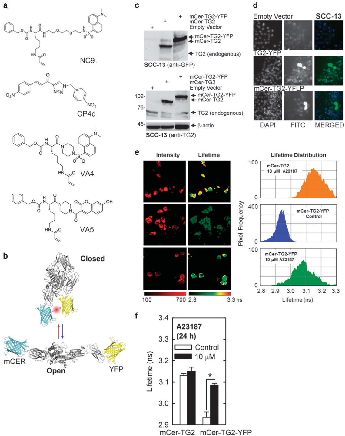
Figure 1. Calcium regulation of TG2 conformation is detected by FRET/FLIM microscopy. (a) Structures of TG2 transamidase site-specific acyl-donor substrate competitive (CP4d) and irreversible (NC9, VA4, VA5) inhibitors. (b) Schematic showing closed and extended TG2 conformations and the position of the mCER (donor) and YFP (acceptor) fluorophores. When TG2 is in the closed/folded conformation, the mCER/YFP fluorophores are closely juxtaposed, resulting in efficient energy transfer. In the TG2 open/extended conformation, separation of the fluorophores results in reduced energy transfer efficiency. (c and d) mCER-TG2 and mCER-TG2-YFP are expressed in SCC-13 cells. Cells were electroporated with 3 μg of each expression plasmid and after 48 h cell extracts were prepared for anti-YFP immunoblot and cells were fixed for anti-YFP cell staining. Note that anti-YFP detects both mCER and YFP. (e) FLIM images of SCC-13 cell electroporated with mCER-TG2 or mCER-TG2-YFP and then treated for 24 h with 10 μM calcium ionophore (A23187). The left panel show mCER donor intensity and the right panel is fluorescent lifetime for a representative experiment. The histogram plot shows the distribution of lifetimes measured in the assayed cells. (f) The average lifetime in nanoseconds was determined for mCER-TG2 or mCER-TG2-YFP expressing cells treated for 24 h with 0 or 10 μM A23187. Differences were determined using the students t -test in this and other experiments. The values are mean ± s.e.m., n = 6 ( P < 0.001).
