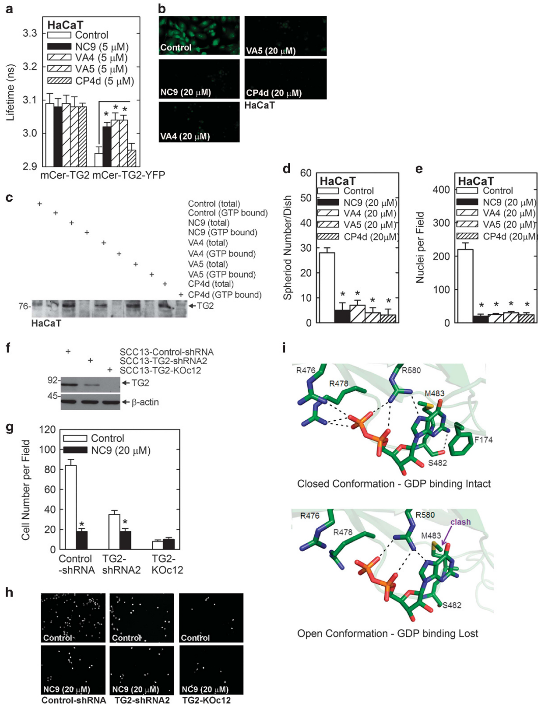
Figure 4. Impact of inhibitors on HaCaT cell biology (a) Inhibitors favour the TG2 open conformation in HaCaT cells. HaCaT cells were electroporated with mCer-TG2 or mCer-TG2-YFP and then treated with 0 or 5 μM of the indicated inhibitor and fluorescent lifetime was monitored. The values are mean ± s.e.m., n = 4 ( P < 0.001 ). (b) Inhibitors suppress TG2 transamidase activity. HaCaT cells were pre-loaded with FC, treated with the indicated inhibitor and then challenged with calcium ionophore, washed and assayed for FC incorporation. (c) Transamidase inhibitors reduce GTP binding to endogenous TG2. HaCaT were incubated for 48 h with the indicated inhibitor and extracts were prepared and incubated with GTP-agarose beads to measure TG2 binding to GTP-agarose. The beads were then washed, boiled in Laemmli buffer and electrophoresed for immunoblot detection of TG2. Cell equivalent quantities of total and bound samples were electrophoresed to facilitate comparison of GTP bound versus total. Similar results were observed in each of three experiments. (d and e) Inhibitors suppress HaCaT cell spheroid formation and matrigel invasion. Experiments were performed as described in Figures 3f and g. The values are mean ± s.e.m., n = 4 ( P < 0.001 ). (f–h) TG2 is required for NC9 action. SCC-13 TG2 knockout cells, and cells expressing wild-type and reduced TG2 levels, were produced using shRNA-mediated knockdown or CRISPR knockout. TG2 level was monitored by immunoblot and ability of the cells to invade a matrigel layer was assessed as previously described. 17,18 This assay measures the ability of cells to pass through a layer of collagen matrix and is a measure of in vivo invasive/metastatic potential. 17 The values are mean ± s.e.m., n = 5 ( P < 0.001 ). The reduced invasion observed in TG2-KOc12 cells does not represent a basal migration rate. Migration can be further suppressed by treatment with agents that target proteins other than TG2 (not shown), but cannot be further suppressed by NC9. (i) Structural analysis of GDP binding at nucleotide binding site in TG2 closed and open conformations (details in text).
